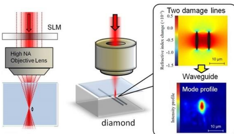
Femtosecond laser writing of NV centers and waveguides
